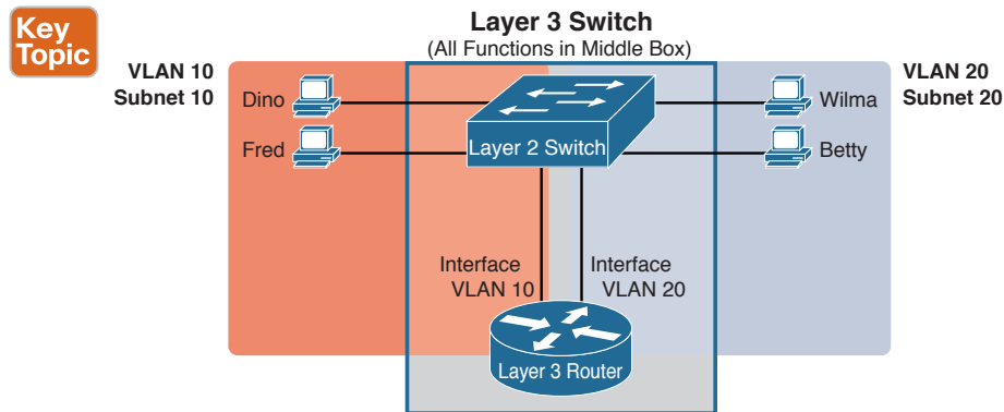
Figure 11-10 Multilayer Switch: Layer 2 Switching with Layer 3 Routing in One Device
