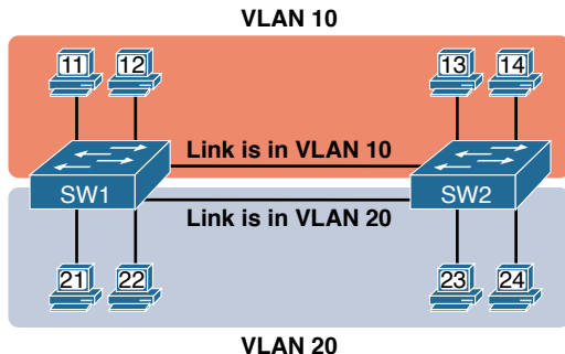
Figure 11-3 Multiswitch VLAN Without VLAN Trunking
