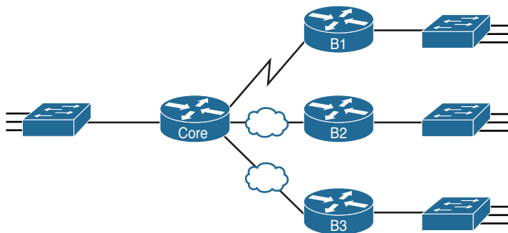
Figure 13-4 Four-Site Internetwork with Small Central Site
