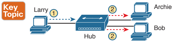
Figure 10-1 10BASE-T (with a Hub): The Hub Repeats Out All Other Ports
