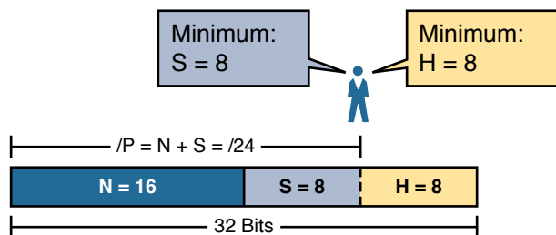
Figure 21-4 One Mask That Meets Requirements
