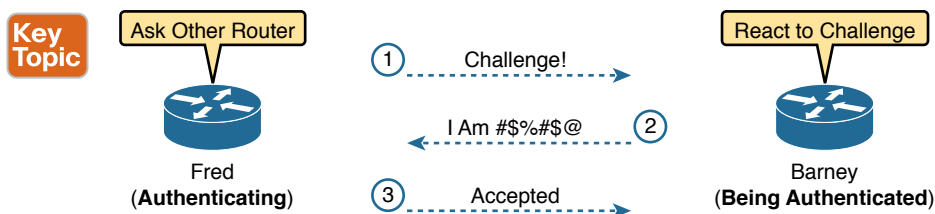
Figure P-14 CHAP Authentication Process
