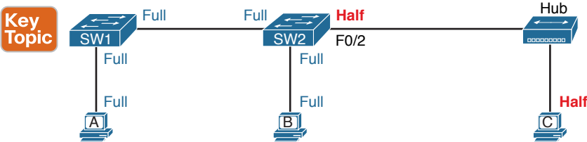
Figure 2-19 Full and Half Duplex in an Ethernet LAN
