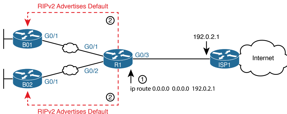
Figure 19-16 A Scenario for RIPv2 to Advertise Default Routes
