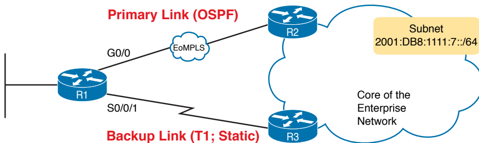
Figure 32-5 Using a Floating Static Route to Key Subnet 2001:DB8:1111:7::/64
