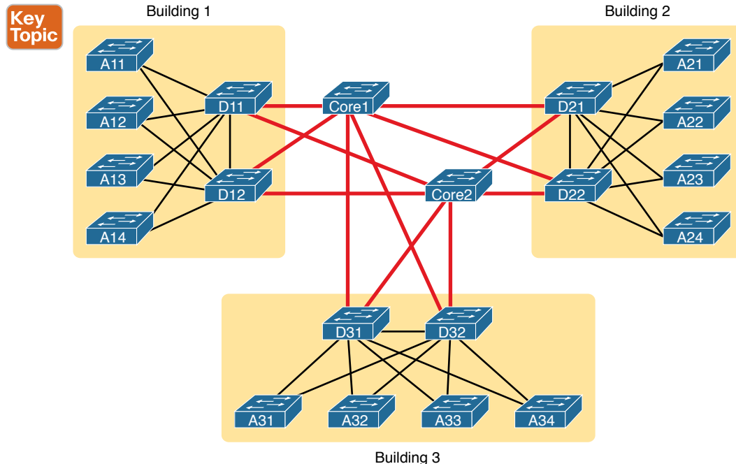
Figure 10-14 Three-Tier Building Design (Core Design), Three Buildings
