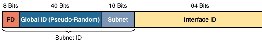
Figure 29-14 IPv6 Unique Local Unicast Address Format
