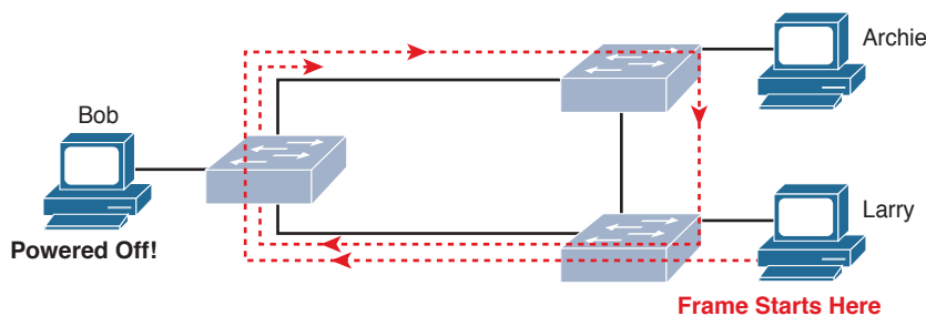
Figure 7-8 Network with Redundant Links but Without STP: The Frame Loops Forever
