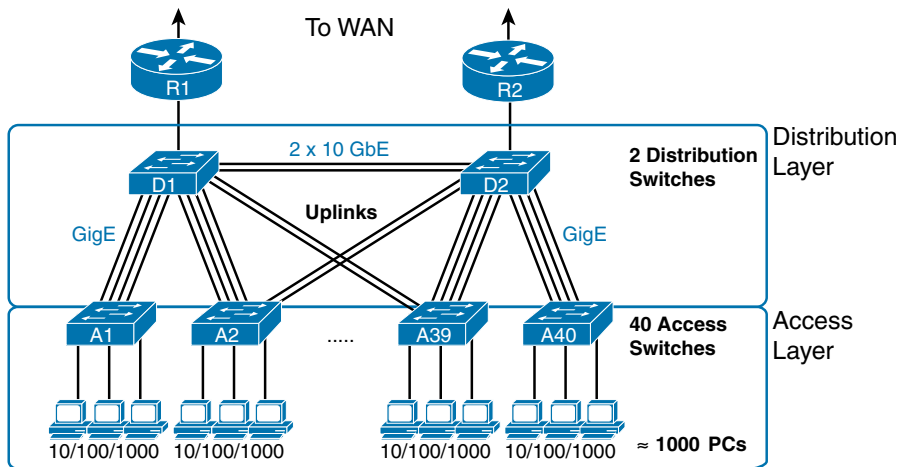
Figure 10-10 Campus LAN with Design Terminology Listed
