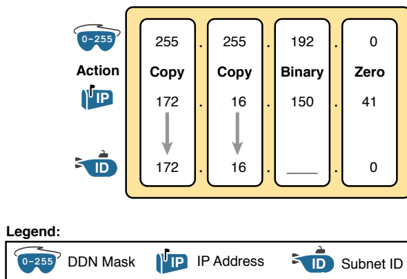
Figure 16-7 Binary Shortcut Example
