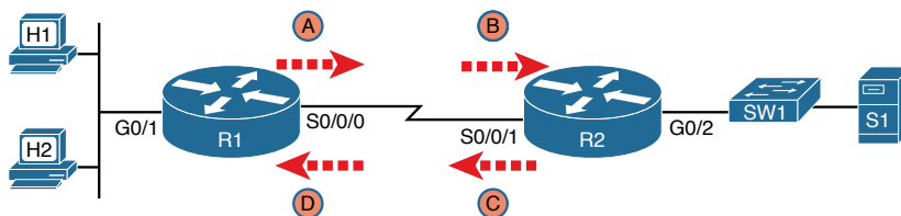
Figure 26-12 Sample Network with IP ACLs in Four Locations
