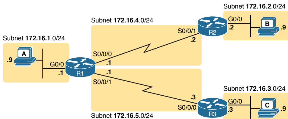
Figure 18-3 IPv4 Network Used to Show Five-Step Routing Example
