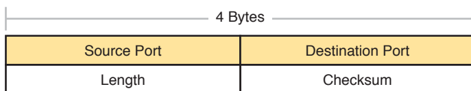
Figure 5-10 UDP Header
